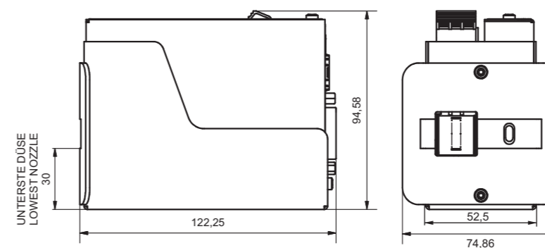
Dimension drawing technical data
